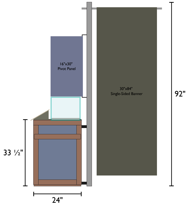
Side View
